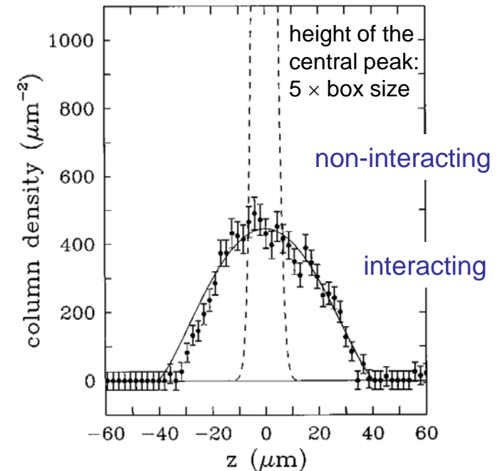
Density distribution of 80000 ^{23}\text{Na} atoms in a trap
