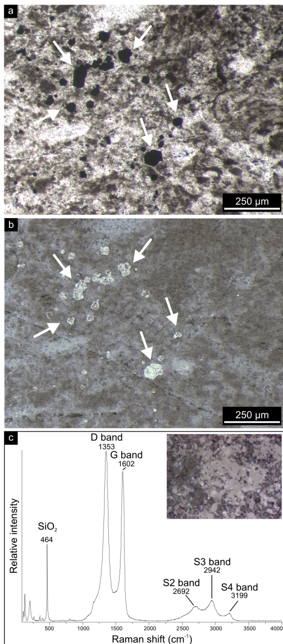
Figure 2. Petrographic observations on the hydrothermal chert vein. (a, b) Thin section photographs ( a transmitted light; b reflected light) showing kerogen (brownish colours) and pyrite (arrows, black colours in a , bright colours in b ) embedded within a fine-grained chert matrix. Note that the pyrite crystals (arrows) are excellently preserved and show no evidence of oxidation. (c) Representative Raman spectrum of kerogen (D band at 1353\text{ cm}^{-1} and G band at 1602\text{ cm}^{-1} ) present in the hydrothermal chert vein. Note the wide D and G bands ( 82 and 55\text{ cm}^{-1} width, respectively), pointing to thermally mature and structurally disordered kerogen, and the absence of an S1 band (at 2450\text{ cm}^{-1} ), consistent with prehnite–pumpellyite to lower greenschist metamorphism and a temperature of ca. 300\text{ }^{\circ}\text{C} (cf. Yui et al., 1996; Delarue et al., 2016).
