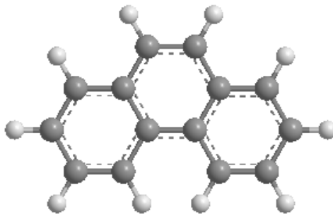
Phenanthrene
