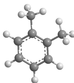
o-Xylene
