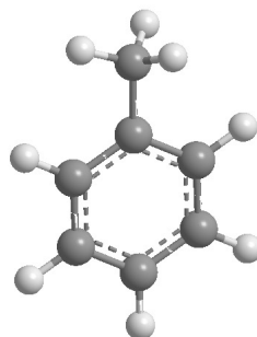
Toluene
