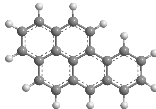
Benzo(a)pyrene
