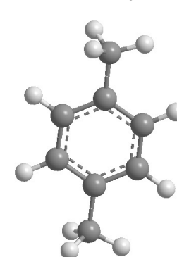
p-Xylene
