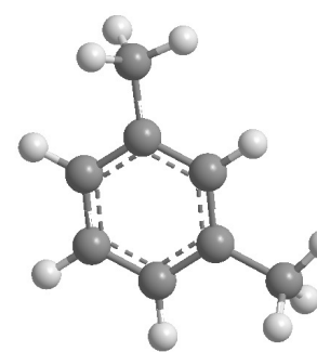
m-Xylene
