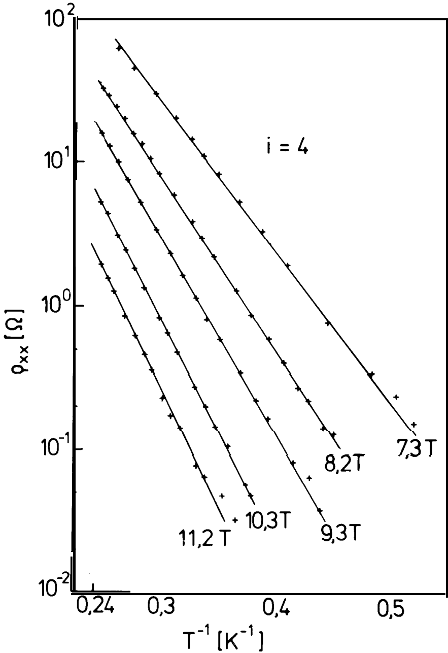
Fig 16. Thermally activated resistivity \rho_{xx} at a filling factor i = 4 for a silicon MOSFET at different magnetic field values.
