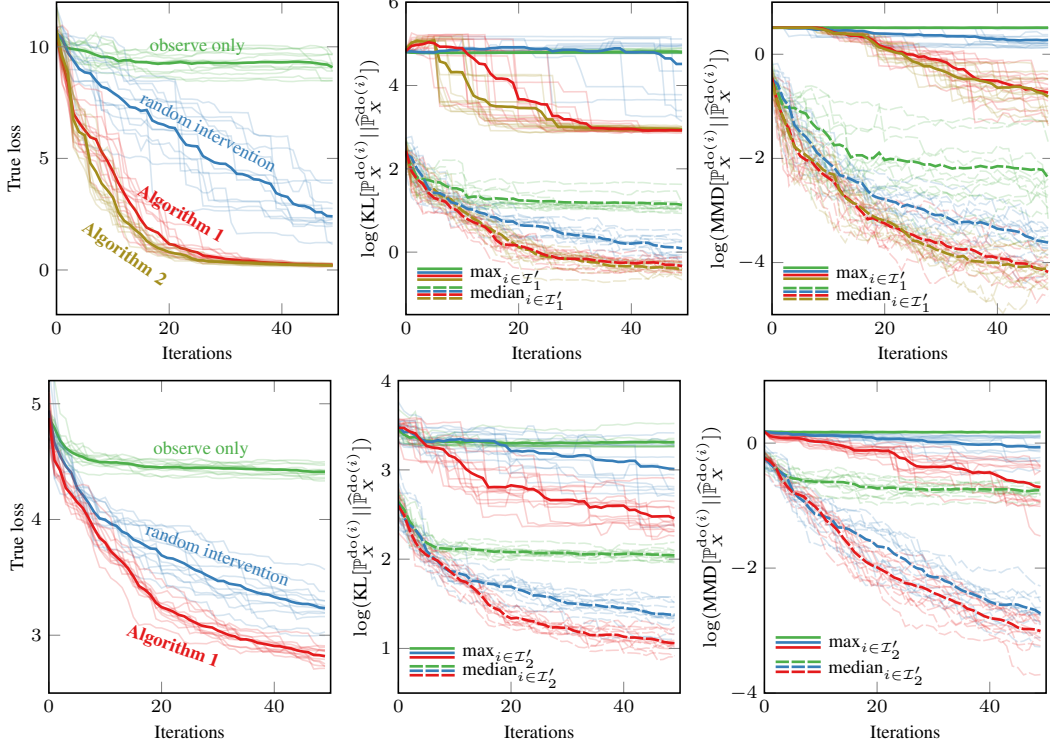
Figure 3: Actively choosing informative interventions speeds up learning. The proposed methods ( Algorithm 1 , Algorithm 2 ) outperform only observing and randomly intervening by each metric of evaluation. Top and bottom row show results of experiments on learning \mathcal{M}_1 and \mathcal{M}_2 respectively. Experimental details described in Section 6. Each experiment was performed many times; faded lines represent results from single trials, bold lines represent averages of these single trials.
