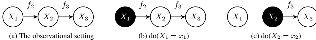
Figure 1: Even in the simple setting of three variables whose graph is a chain, there is a non-trivial trade-off between the information one expects to gain by performing different interventions (see text).
