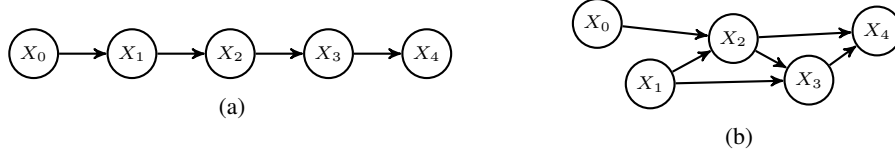
Figure 2: The causal graphs of the SCMs (a) \mathcal{M}_1 and (b) \mathcal{M}_2 used in the experiments (Section 6).
