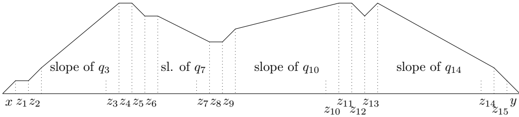
■ Figure 4 Example for positions of z_1, \dots, z_{15} fitting to the input word.
