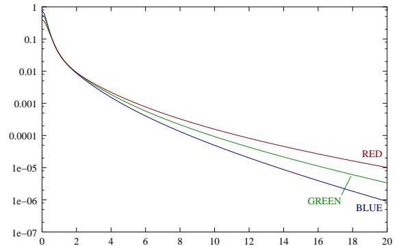
Figure 2: The BSSRDF model (from 11 ) used in this paper. Constants for some materials are also found in 11 . The graphs show the diffuse reflectance due to subsurface scattering \mathbf{R}_d for a measured sample of marble with \sigma'_s = (2.19, 2.62, 3.00)^{(*)} , \sigma_a = (0.0021, 0.0041, 0.0071)^{(*)} and \eta = 1.5 . \mathbf{R}_d(\mathbf{r}) indicates the radiosity at a distance r in a plane, due to unit incident power at the origin. Subsurface scattering is significant up to a distance of several millimeters in marble. The graphs also explain the strong color filtering effects observed at larger distances.
