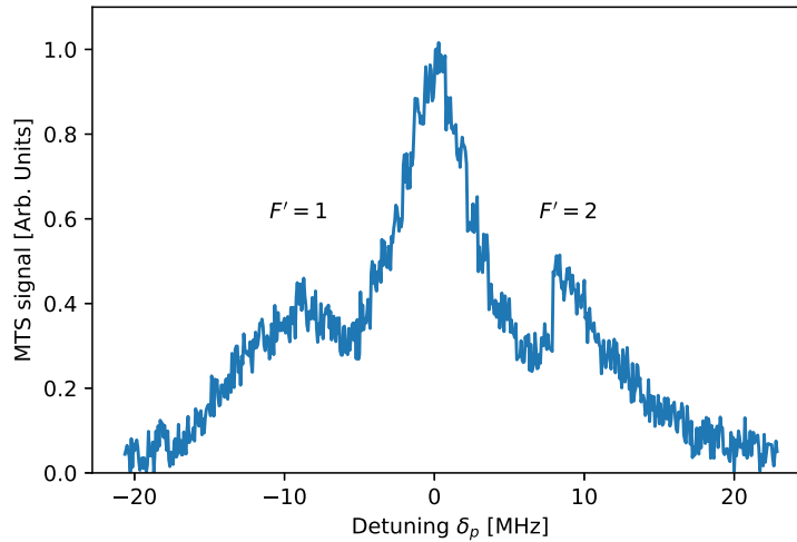
Figure 6.12: Probe beam MTS signal \zeta(\delta_p) as a function of shared probe and pump beam detuning \delta_p . Approximate Rabi frequencies are \Omega_{probe} = 10\text{MHz} and \Omega_{pump} = 5\text{MHz} . The scan is obtained using a chopping frequency of 250 kHz and a vapour cell temperature of 125^\circ\text{C} .
