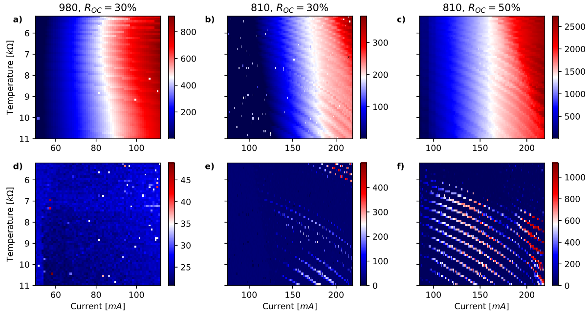
Figure 3.7: I, T -stability maps of photodiode voltage of DC (a), (b), (c) and AC (d), (e), (f) components for the 980B ECDL (a), (d) and a 810A ECDL with a 30% (b), (e) and 50% (c), (f) outcoupler. The DC signal scales linearly to laser output power, whereas the AC signal is the sum of all Fourier components between f_{min} = 4 \text{ Hz} and f_{max} = 40 \text{ kHz} . The inverse temperature is given as the resistance of the thermistor of the ECDL: the minimum (maximum) resistance R_{min} ( R_{max} ) corresponds to a temperature of 37^\circ\text{C} ( 21^\circ\text{C} ).
