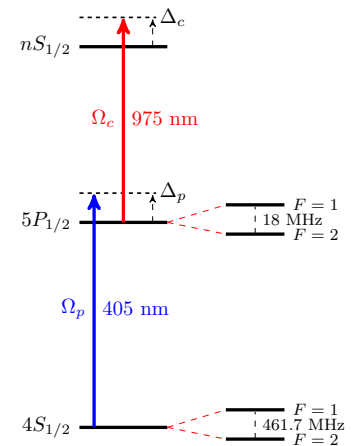
Figure 6.1: The three-level system in scope, where the levels are coupled with Rabi frequencies \Omega_p and \Omega_c and blue detuned by \Delta_p and \Delta_c .
