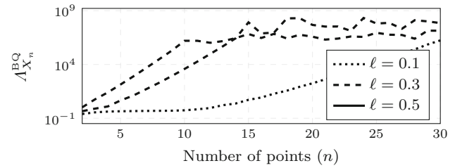
Fig. 4 Bayesian quadrature stability constants for the Gaussian kernel (12) with different length-scales, the uniform measure on [0, 1] and n points uniformly placed on this interval (end points not included). The levelling off appears to be caused by loss of numerical precision
