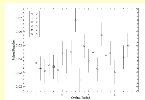
Figure 3: Pulsed fraction values for 6 orbital phases indicated by different symbols for all the four orbits in the 0.5-3.0 keV energy band.
