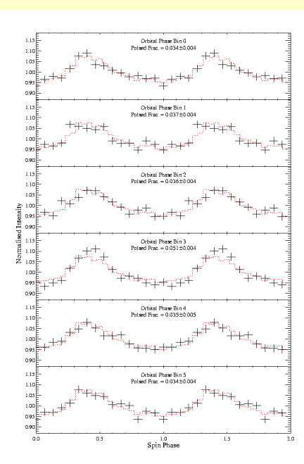
Figure 2: Folded light curves of XTE J1807-289 at different orbit phases in the energy range 0.5-10 keV. Orbit phase 0 relates to t_0 - 44.08 s
