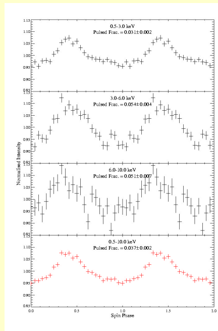
Figure 1: Folded spin light curves of XTE J1807-289 in different energy ranges. From top to bottom: 0.5-3.0, 3.0-6.0, 6.0-10.0 and 0.5-10 keV. The pulse profile is shown twice for clarity
