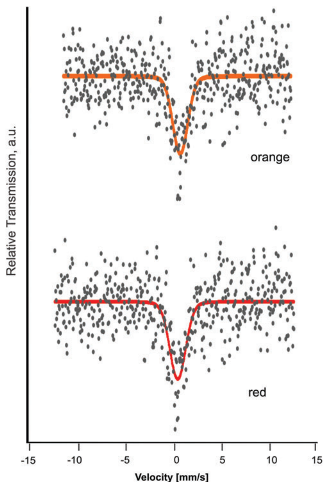
FIG. 5. ^{57}\text{Fe} Mössbauer spectroscopy of orange and red samples of Lake Whurr at 5 K after digestion in 6 M anoxic HCl at 70°C for 24 h. Shown are the raw data (gray) and the sum of fits (orange/red). a.u. = arbitrary units. (Color graphics available at www.liebertonline.com/ast )
