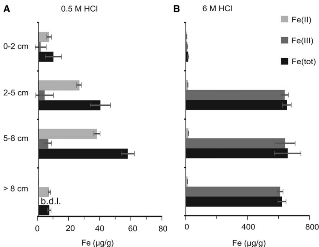
FIG. 2. Concentrations of different Fe fractions in a sediment profile of Lake Orr in \mu\text{g/g} dry sediment. (A) 0.5 M HCl extractable (“poorly crystalline”) Fe. (B) 6 M HCl extractable (“crystalline”) Fe. Error bars give standard deviations from duplicate measurements. b.d.l. = below detection limit.
