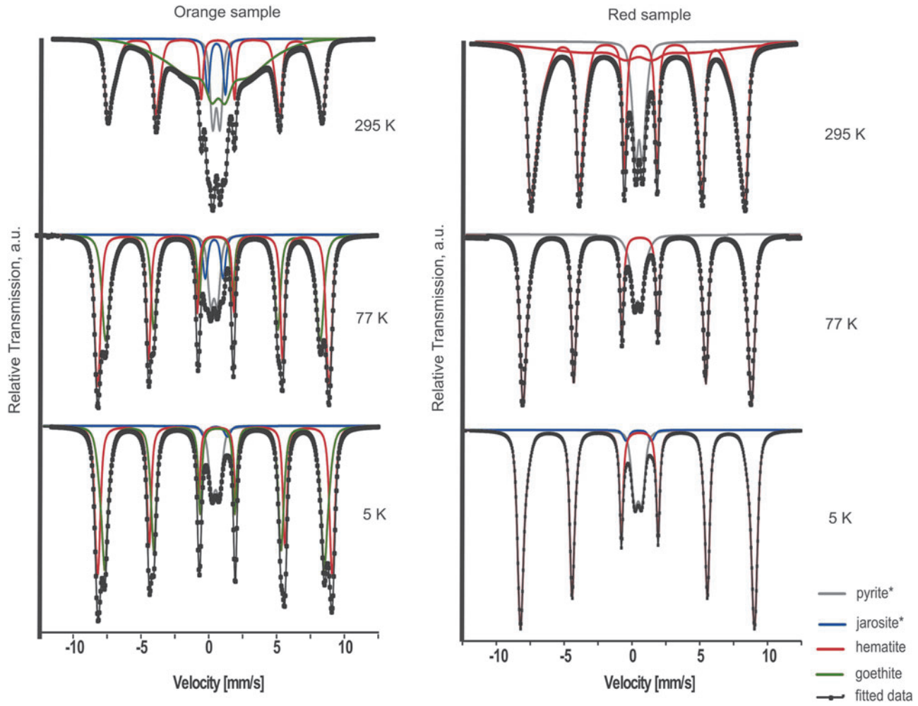
FIG. 4. ^{57}\text{Fe} Mössbauer spectroscopy of orange and red samples of Lake Whurr sediments at temperatures of 295, 77, and 5 K. *indicates the tentative identification of pyrite and jarosite. a.u. = arbitrary units.
