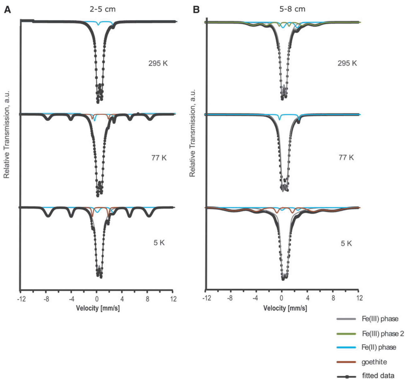
FIG. 6. ^{57}\text{Fe} Mössbauer spectroscopy of samples from (A) 2–5 cm and (B) 5–8 cm depth of Lake Orr sediments at temperatures of 295, 77, and 5 K. a.u. = arbitrary units.
