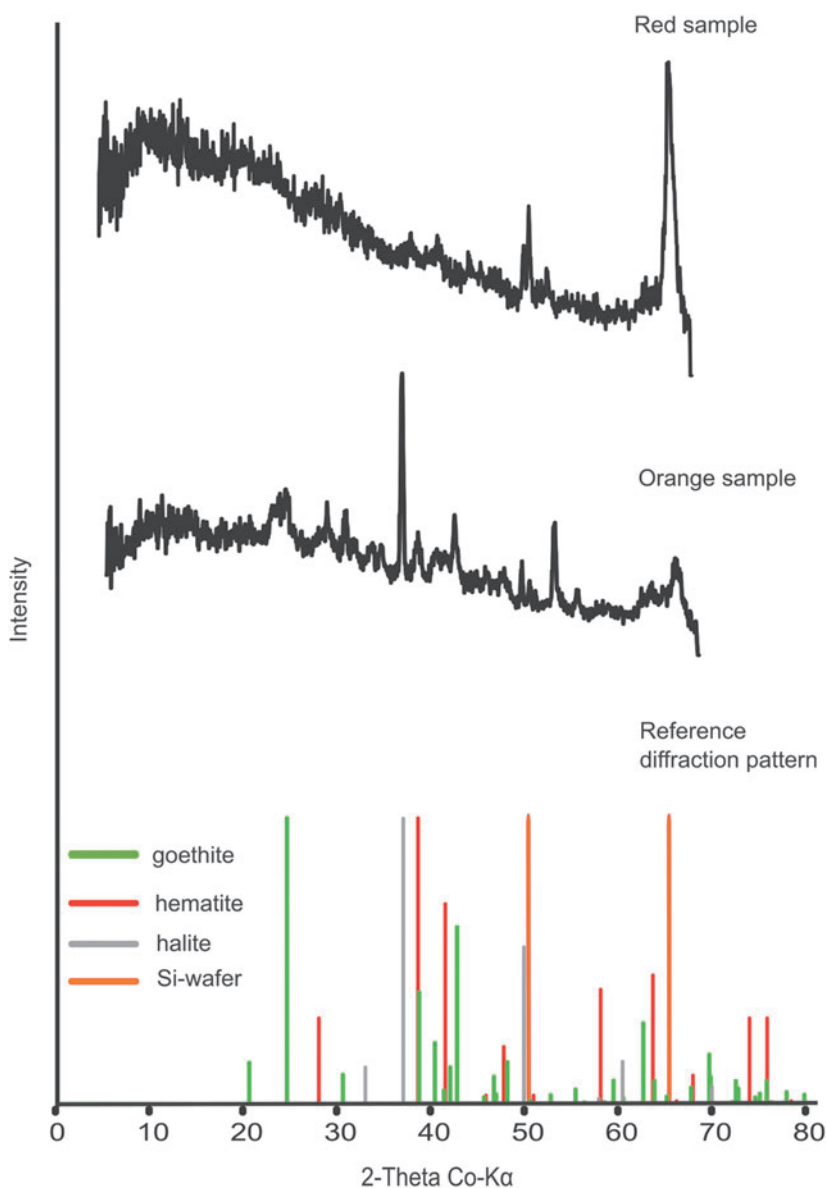
FIG. 3. X-ray diffraction pattern of red and orange samples from Lake Whurr sediments. The bottom panel shows reference diffraction patterns of goethite, hematite, and halite and a diffraction pattern of the Si wafer.
