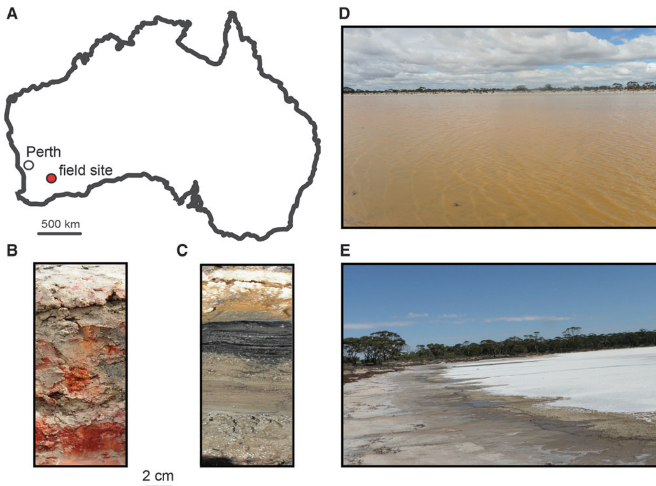
FIG. 1. Location of the field site in Australia (A), sediment characteristics of Lake Whurr 2013 (B) and Lake Orr 2012 (C), and differences in the appearance of Lake Whurr after rain events in the Australian autumn of 2013 (D) and desiccated bed of Lake Orr in autumn 2012 (E).
