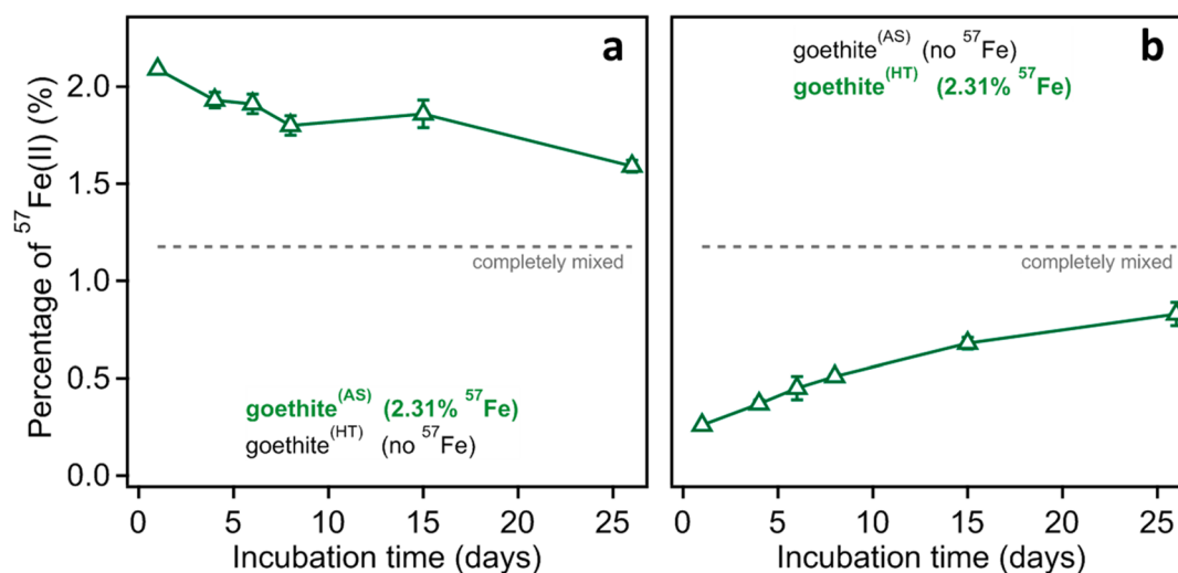
Figure 1. Percentage of ^{57}\text{Fe} isotope in reduced iron (Fe(II)) from reactors containing a labeled mix of goethite (AS) and goethite (HT) . In panel a, goethite (AS) is labeled with the ^{57}\text{Fe} isotope, while in panel b, goethite (HT) is labeled with the ^{57}\text{Fe} isotope. Data corresponds to an average of biological triplicates, and the error bars indicate standard deviations. Experimental conditions: 10^8 cells \text{mL}^{-1} Geobacter sulfurreducens ; 10 \mu\text{M} AQDS; (a) 1 \text{ g L}^{-1} ^{56}\text{Fe} -goethite (AS) + 1 \text{ g L}^{-1} ^{57}\text{Fe} -goethite (HT) or (b) 1 \text{ g L}^{-1} ^{57}\text{Fe} -goethite (AS) + 1 \text{ g L}^{-1} ^{56}\text{Fe} -goethite (HT) .
