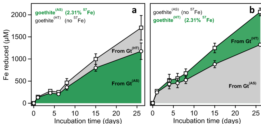
Figure 2. Origin of the reduced iron (Fe(II)) based on isotope signature and concentration of the microbially reduced Fe from reactors containing a labeled mix of goethite (AS) and goethite (HT) . Data corresponds to an average of biological triplicates, and the error bars indicate standard deviations. Experimental conditions: 10^8 cells \text{mL}^{-1} Geobacter sulfurreducens ; 10 \mu\text{M} AQDS; (a) 1 \text{ g L}^{-1} ^{56}\text{Fe} -goethite (AS) + 1 \text{ g L}^{-1} ^{57}\text{Fe} -goethite (HT) or (b) 1 \text{ g L}^{-1} ^{57}\text{Fe} -goethite (AS) + 1 \text{ g L}^{-1} ^{56}\text{Fe} -goethite (HT) .
