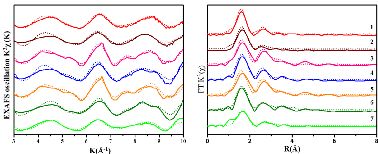
Figure 5. Cr K-edge EXAFS signals weighted by (A) k^3 spectra and the (B) radial distribution function of Cr-loaded samples. (1) 2 mM Fe+ 1 g L -1 BC at pH 7; (2) 10 mM Fe+ 0.5 g L -1 BC at pH 5; (3) 10 mM MNP+ 0.5 g L -1 BC at pH 7; (4) 10 mM MNP at pH 5; (5) 10 mM MNP at pH 7; (6) 1 g L -1 BC at pH 3 and (7) 1 g L -1 BC at pH 2. Solid lines represent experimental data and dotted lines represent fit, respectively.
