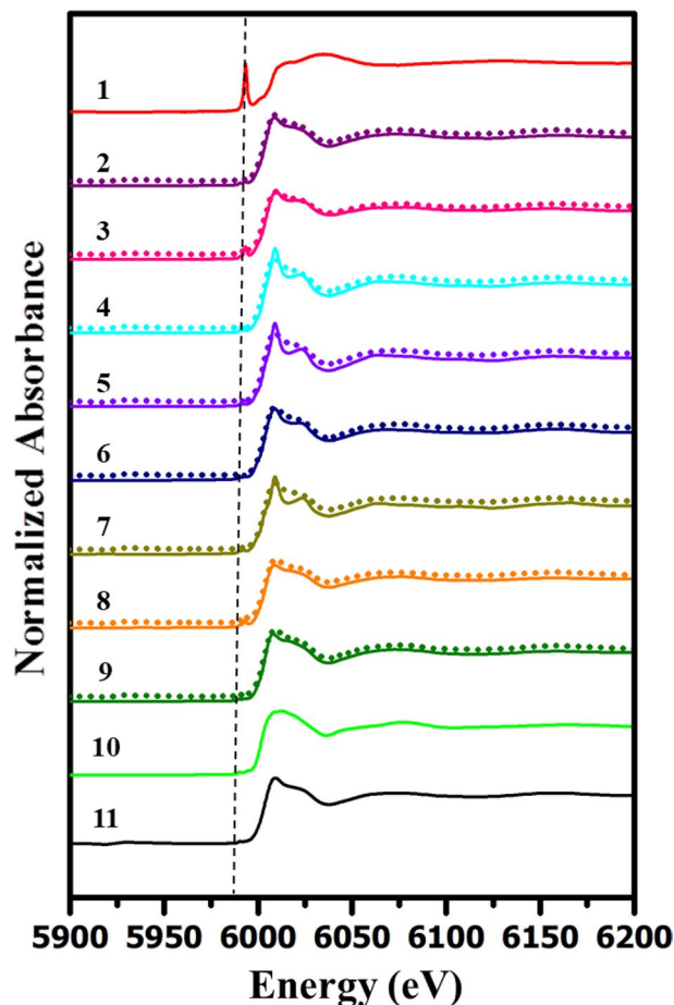
Figure 4. Cr K-edge XANES spectra of chromium references and Cr-loaded MNP-BC, MNPs and BC at different pH conditions (1) K_2Cr_2O_7 standard; (2) 2 mM Fe+ 1 g L -1 BC at pH 7; (3) 4 mM Fe+ 1 g L -1 BC at pH 5; (4) 10 mM Fe+ 0.5 g L -1 BC at pH 5; (5) 10 mM MNP+ 0.5 g L -1 BC at pH 7; (6) 10 mM MNP at pH 5; (7) 10 mM MNP at pH 7; (8) 1 g L -1 BC at pH 3; (9) 1 g L -1 BC at pH 2; (10) Cr(III) acetate standard and (11) Cr(OH) 3 standard. Solid lines represent experimental data and dotted lines represent fit, respectively.
