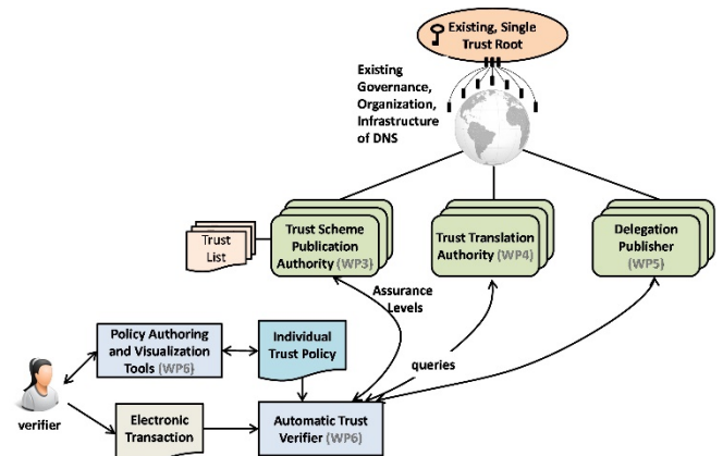
Figure 1: The LIGHTest Reference Architecture (see also [1], [2])
