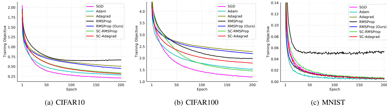
Figure 6. Training Objective vs Number of Epoch for 4-layer CNN
