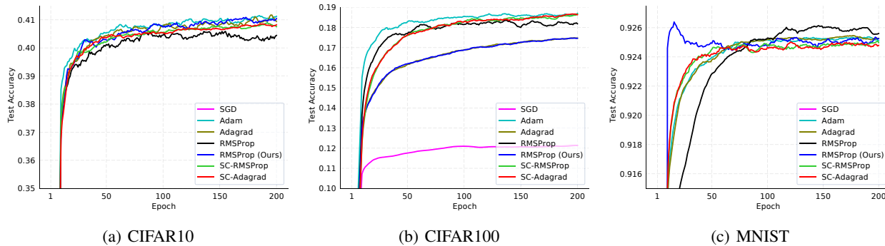
Figure 5. Test Accuracy vs Number of Epochs for L2-Regularized Softmax Regression
