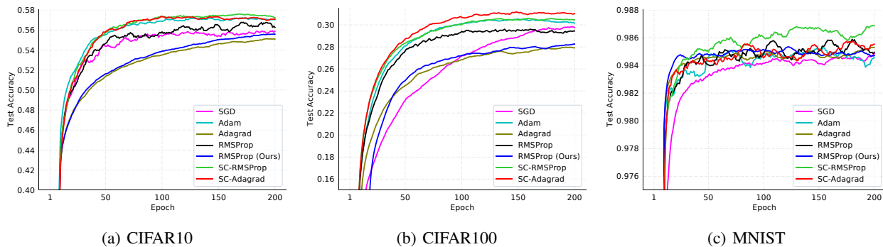
Figure 8. Test Accuracy vs Number of Epochs for 3-layer MLP
