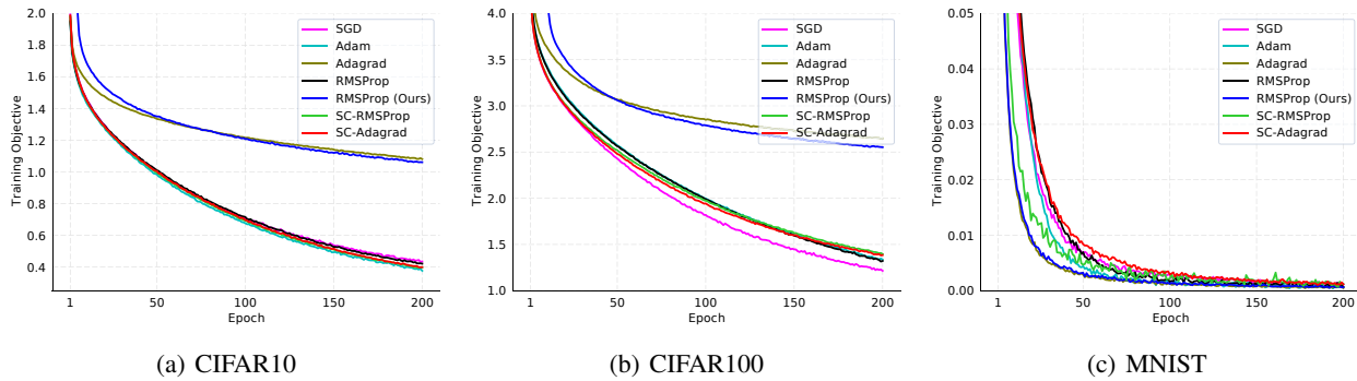
Figure 7. Training Objective vs Number of Epoch for 3-layer MLP
