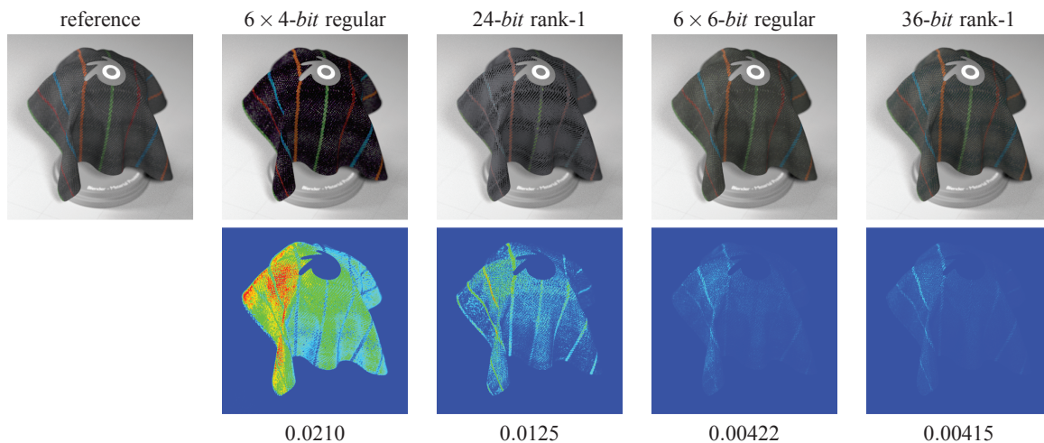
Figure 4: This figure shows the result of quantizing a 6d spectral reflectance texture to 24-bit and to 36-bit using a regular grid and a rank-1 lattice. The second row shows the difference to the reference image and the last row the root mean square error of the quantized texture data. The input data have a resolution of 832 \times 669 \times 6 (12.7 MB) and the quantization results in 1.6 MB and 2.1 MB, respectively.
