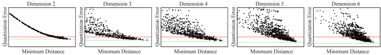
Figure 2: Correlation between minimum distance and quantization error plotted for dimensions 2–6. Each dot in the plots represents the minimum distance and quantization error of an s -dimensional rank-1 lattice with 1024 points, where the generator vector is chosen at random. In all plots the y -axis (quantization error) covers the range [0.07, 0.14] . Note that both axes are at logarithmic scale. The red line shows the quantization error for the Cartesian lattice \mathbb{Z}^s (always 0.08333) and the green line the quantization error for the best known lattice quantizer for the corresponding dimension (compare this also to Table 1). The quantization error of the rank-1 lattice was computed via Monte Carlo integration. It can be seen that maximizing the minimum distance of a rank-1 lattice leads to a small quantization error.
