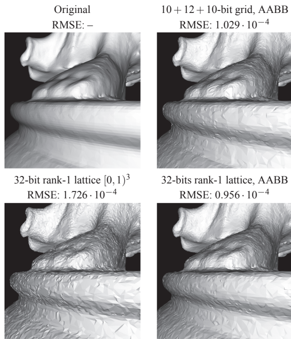
Figure 5: Stanford Buddha quantized to 32-bits per vertex. The configuration of 10 + 12 + 10-bits is optimal for regular grid quantization of this model. However, rank-1 lattice quantization shows better results than the regular grid when optimized for the axis-aligned bounding box. Finding the parameters for this lattice took about 2 min with the python implementation of the search algorithm. RMSE, root mean square error.
