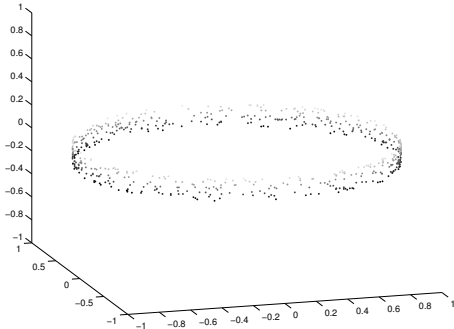
Figure 2. 600 samples of the circle with uniform noise of height 0.1 in the z -direction
