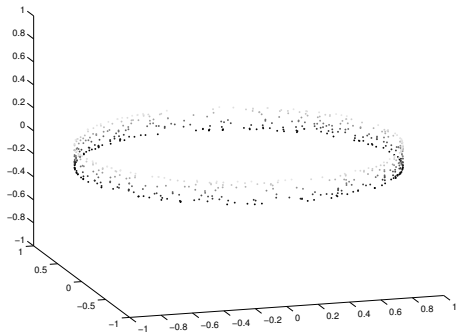
Figure 1. 600 samples of the sinusoid
