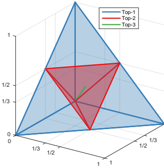
Figure 2: Top- k simplex \Delta_k(1) for m = 3 . Unlike the standard simplex, it has \binom{m}{k} + 1 vertices.
