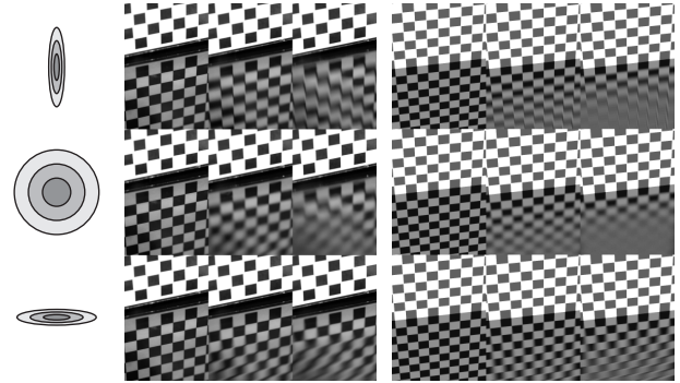
Figure 8: Photos of Setup 1 (left, checkerboard pitch 10 mm) and raytraced simulations (right) of various degrees of anisotropic blur.
