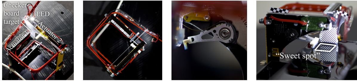
Figure 6: Various views of Setup 2 built from a pair of discarded 2.5-inch hard disk drives. From left to right: Components, top view, close-up on actuator 2, water surface and checkerboard target.
