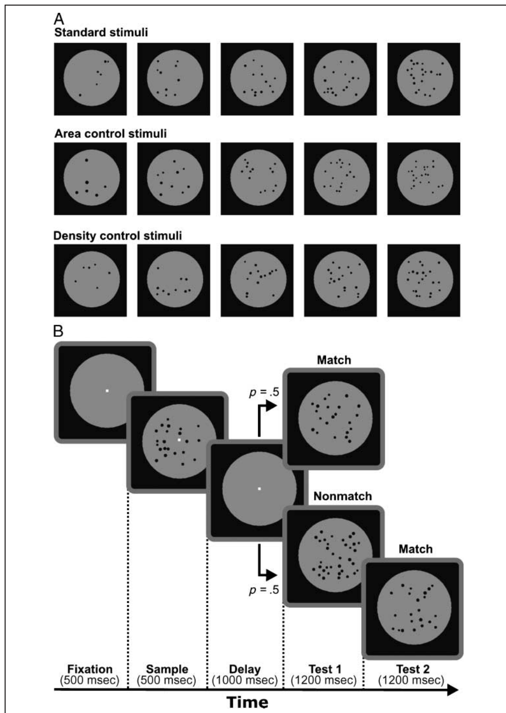
Figure 1. Delayed match-to-numerosity protocol and example stimuli. (A) Example stimuli (standard, area control, and density control) for sample numerosity 14, which had to be discriminated from numerosities 6, 10, 18, and 22. (B) A trial started when the monkey grabbed the bar and fixated the fixation spot. A sample stimulus (here, 22 dots) was followed by a delay period. The test stimulus contained either the same number of items (“match”) or a different quantity of dots (here, 35 dots) (“nonmatch”). Each nonmatch stimulus was followed by a match stimulus, with the same set size as the sample. When a match stimulus appeared, the monkey was required to release the lever to receive a reward.
