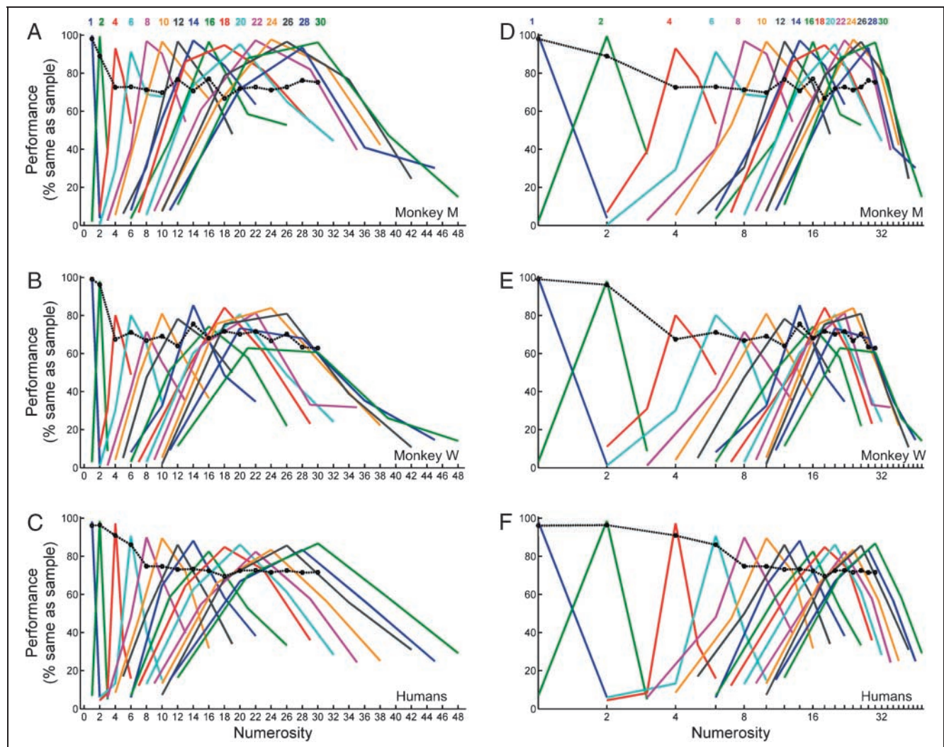
Figure 5. Scaling of performance distributions for human and monkey subjects. Same layout as in Figure 2. The behavioral tuning curves were plotted on linear [(A) Monkey M, (B) Monkey W, (C) humans] and logarithmic scales [(D) Monkey M, (E) Monkey W, (F) humans].
