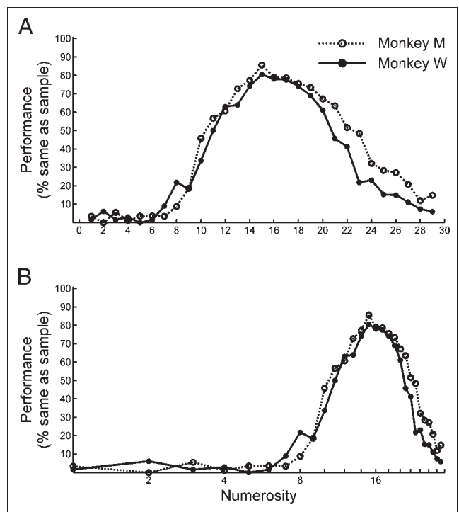
Figure 6. Detailed discrimination performance functions of both monkeys for sample numerosity 15. The functions are plotted on (A) a linear and (B) a logarithmic scale.
