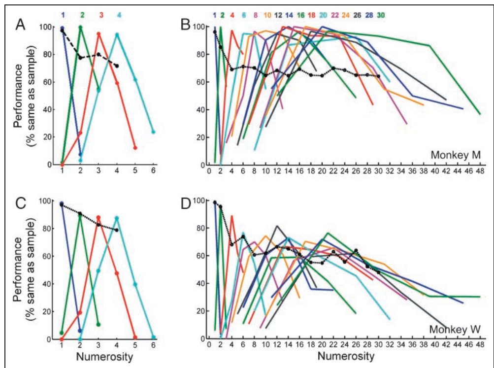
Figure 2. Behavioral tuning curves derived from the monkeys' performance to the broad range of numerosities. The functions reflect the probability that a monkey judged displays in the test period as containing the same number of items as the sample numerosity. The data point at the center of each colored function indicates the correct performance in the match trials for the sample numerosities (shown in the same color above each curve). The data points to the left and the right of the center reflect performance in the nonmatch trials (i.e., where the first test display showed a smaller or larger number of items), presented as the percentage of errors for the respective nonmatch numerosity. (A) Monkey M's and (C) Monkey W's performance curves for the task with small numerosities (1 to 4). (B) Monkey M's and (D) Monkey W's filter functions for the spontaneous transfer from the discrimination of small numerosities to the discrimination of large numerosities.
