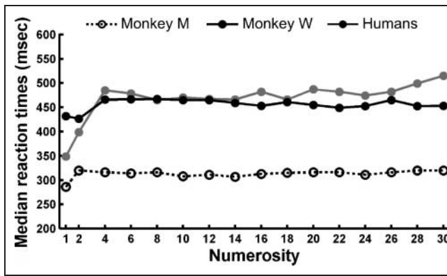
Figure 8. Median reaction times for all tested numerosities (only correct match trials).
