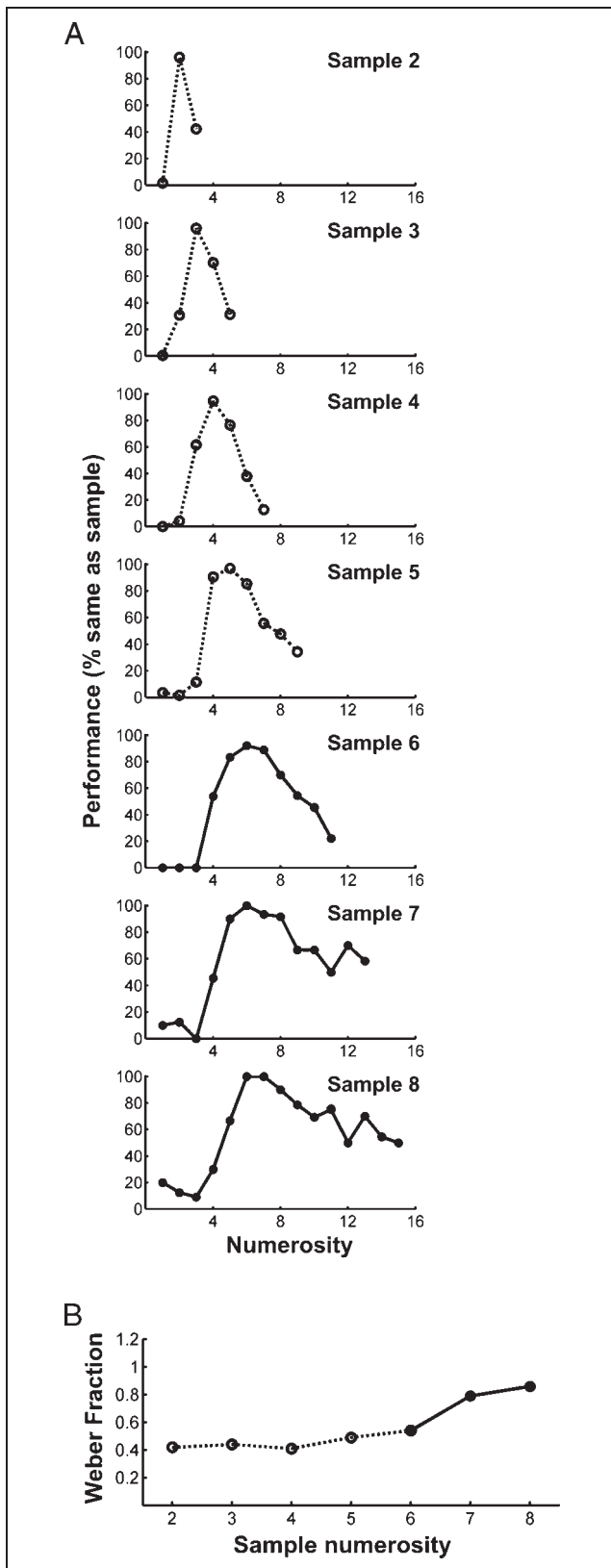
Figure 3. Monkey W's discrimination performance in the transfer trials experiment. (A) Discrimination filter functions for previously trained, small numerosities (dotted line) and new, larger numerosities (solid line). (B) Weber fractions for reinforced discriminations and transfer tests.
