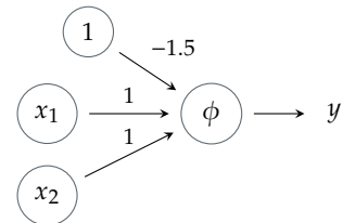
Figure 4.5: Example of an AND gate as a neural network. Using the binary step function as the activation function \phi , we can build an AND gate for the inputs x_1 and x_2 . Setting the bias, as well as the network weights for both inputs to 1 and the weight of the bias to -1.5 the output y of the node is equivalent to an AND gate. If instead the weight of the bias term were set to -0.5 , the node would turn into an OR gate.
