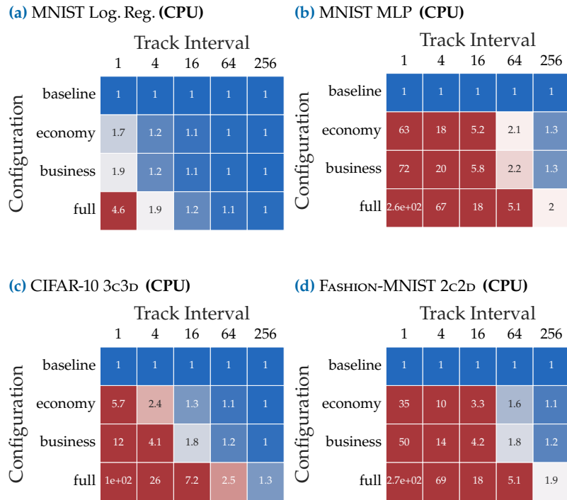
Figure C.9: Overhead of COCKPIT configurations on CPU for four different problems with varying tracking interval. Color bar is the same as in Figure 7.6.
