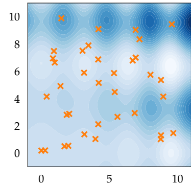
Figure 3.9: Illustration of random search. In total, 36 random samples (✕) are drawn uniformly. Compared to grid search, more different values for each hyperparameter are tested.
