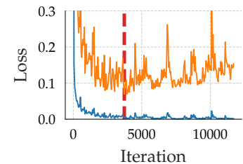
Figure 2.12: Early stopping can be used to prevent overfitting. The training loss (—) of a simple convolutional neural network on MNIST decreases as training progresses. The test loss (—) initially decreases as well but at some point plateaus and even begins to increase again. Stopping training earlier, at the point of minimal test loss (- -), can provide a solution with better generalization capabilities. Note that due to the stochastic nature of the training process, both loss curves are noisy.
