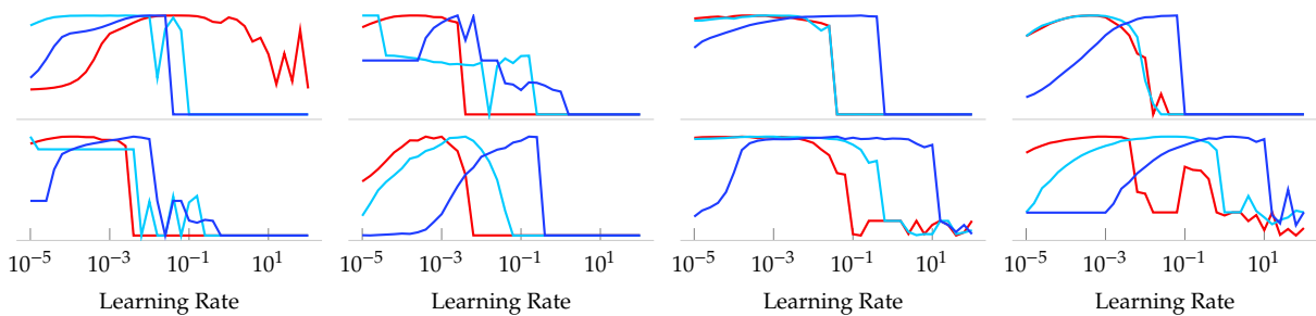
Figure 5.3: Relative performance against learning rate for each test problem and optimizer. Top row shows test problems P1 to P4, bottom row the test problems P5 to P8. The optimizers are represented in the same color as in Figure 5.2 and throughout this thesis, where ● represents SGD, ● represents MOMENTUM, and ● the ADAM optimizer.
