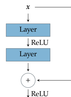
Figure 4.13: Illustration of a residual connection.
