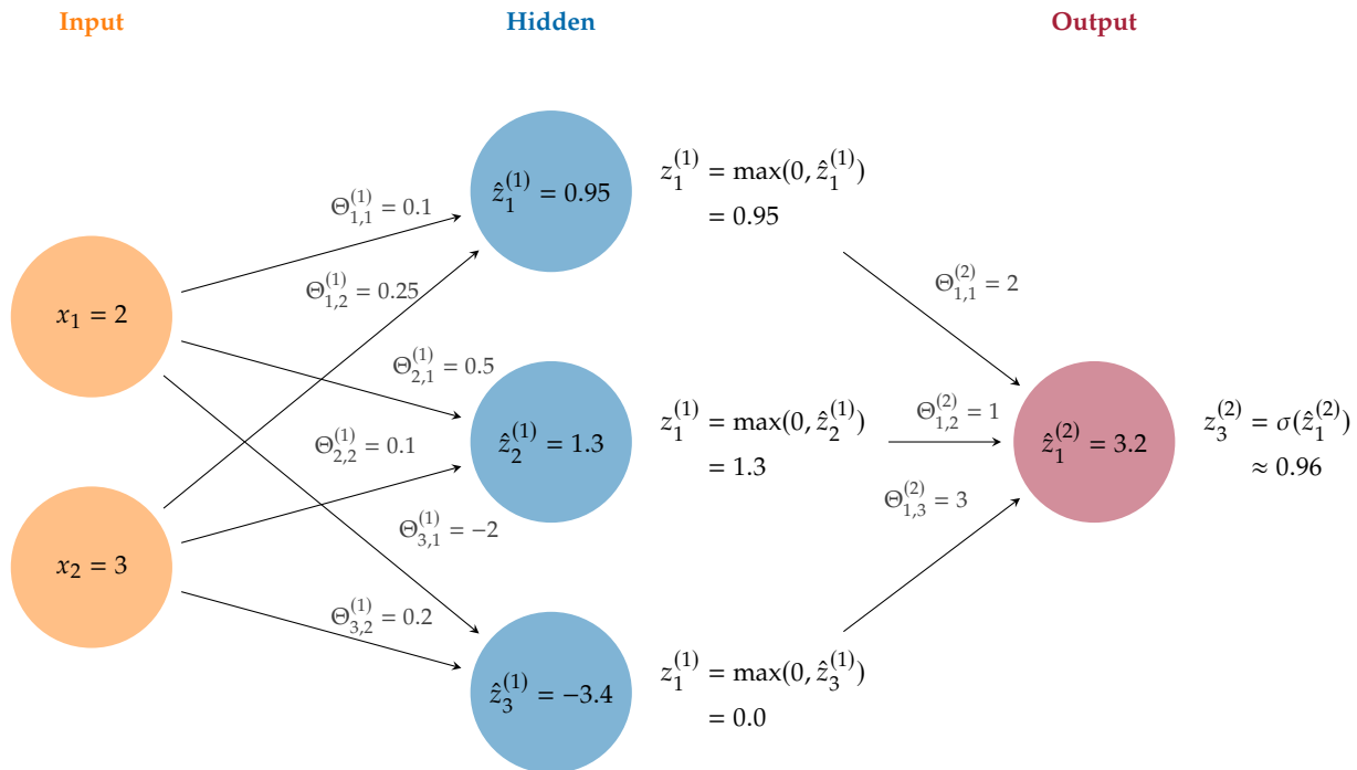
Figure 4.1: Illustration of a very simple neural network with nine parameters. Information “flows” from the input nodes (●) via the hidden nodes (●) to the output nodes (●). The inputs x = (2 \ 3)^T could, for instance, be the (vectorized) pixel values of an image which should be classified. In this architecture, the input values are broadcast to all neurons in the hidden layer, which compute a weighted sum of all incoming signals. The current weights are denoted along the connection ( \rightarrow ), e.g. \Theta_{3,2}^{(1)} = 0.2 represents that the third neuron in the hidden layer, weights the second input by 0.2. The result of the weighted sum, the pre-activation, is denoted in the node. Crucially, a non-linear activation function is applied, which for the hidden layer in this example is simply the ReLU function, i.e. \max(0, \hat{z}) , where \hat{z} is the pre-activation. The result after the activation is written to the right of the neuron. A single output neuron weights the outputs of the hidden neurons and applies another activation function, this time a sigmoid. The output of the network for this example is 0.96 which could, for instance, represent the probability that the given image contains a hot dog.
