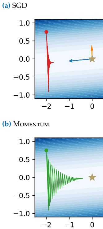
Figure 3.6: Illustration of the difference between SGD and Momentum. (a) On a two-dimensional deterministic quadratic loss function with one high-curvature (→) and one low-curvature direction (→) SGD (—) oscillates heavily without much progress towards the minimum (★). (b) Momentum (—) accumulates “velocity” in the low-curvature direction and thus progresses much more towards the minimum compared to SGD.
