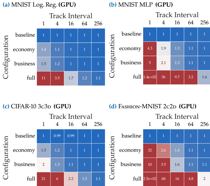
Figure C.8: Overhead of COCKPIT configurations on GPU for four different problems with varying tracking interval. Color bar is the same as in Figure 7.6.
