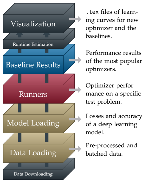
Figure 5.1: Illustration of the different steps implemented in the DEEPOBS package and their outputs. The color of each block highlights the way a user mostly interacts with this part. Blocks in ● signify classes, those in ● are used via command line scripts. ● signals data packaged with DEEPOBS and ● denotes parts provided through template scripts.
