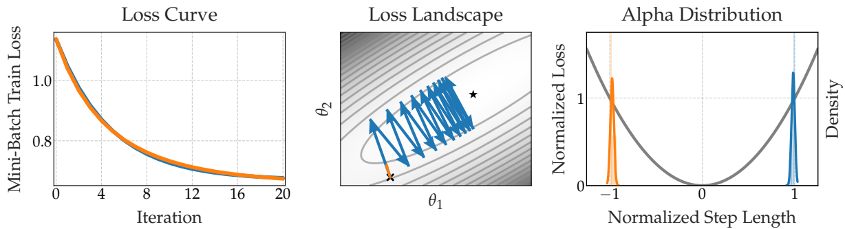
Figure 7.1: Illustrative example: Learning curves do not tell the whole story. Two different optimization runs (— / —) can lead to virtually the same loss curve ( left ). However, the actual optimization trajectories ( center ), exhibit vastly different behaviors. In practice, the trajectories are intractably high-dimensional and cannot be visualized directly. Recommendable actions for both scenarios (increase/decrease the learning rate) cannot be inferred from the loss curve alone. The Alpha distribution, one of COCKPIT’s instruments ( right ), not only clearly distinguishes the two scenarios, but also allows for taking decisions regarding how the learning rate should be adapted. See Section 7.3.3 for further details.
