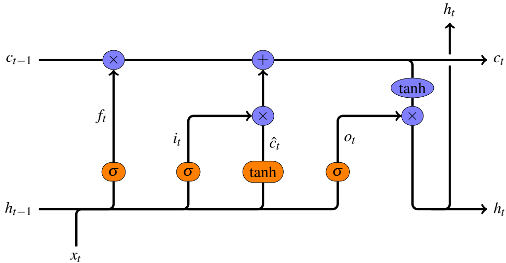
Figure 3 A long short-term memory (LSTM) network. The orange nodes represent neural network layers: matrix multiplication by a weight matrix (plus addition of bias) before a point-wise nonlinearity as labeled. The blue nodes represent pointwise application of a function. The merging of two arrows represents vector concatenation and the splitting of an arrow represents copying.
