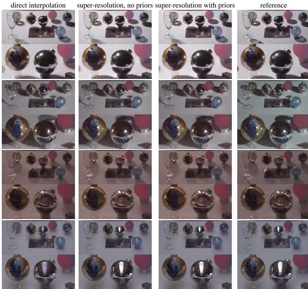
Figure 9: Results of a complex scene with detail zoom-ins for renderings in two point light conditions (upper four rows) and in the Galileo's Tomb and Uffizi environment maps [Deb98]. The super-resolution reflectance field is upsampled from 230 to 3547 images, the reference has 14116 images. Our upsampling approach produces superior results compare to linear interpolation. Applying the regularization (second column from the right) further improves shadow boundaries; for real-world illuminations, the non-regularized version is already close in quality. Note that the reference exposes aliasing which the super-resolution images do not show due to sub-pixel blurring during the upsampling steps.
