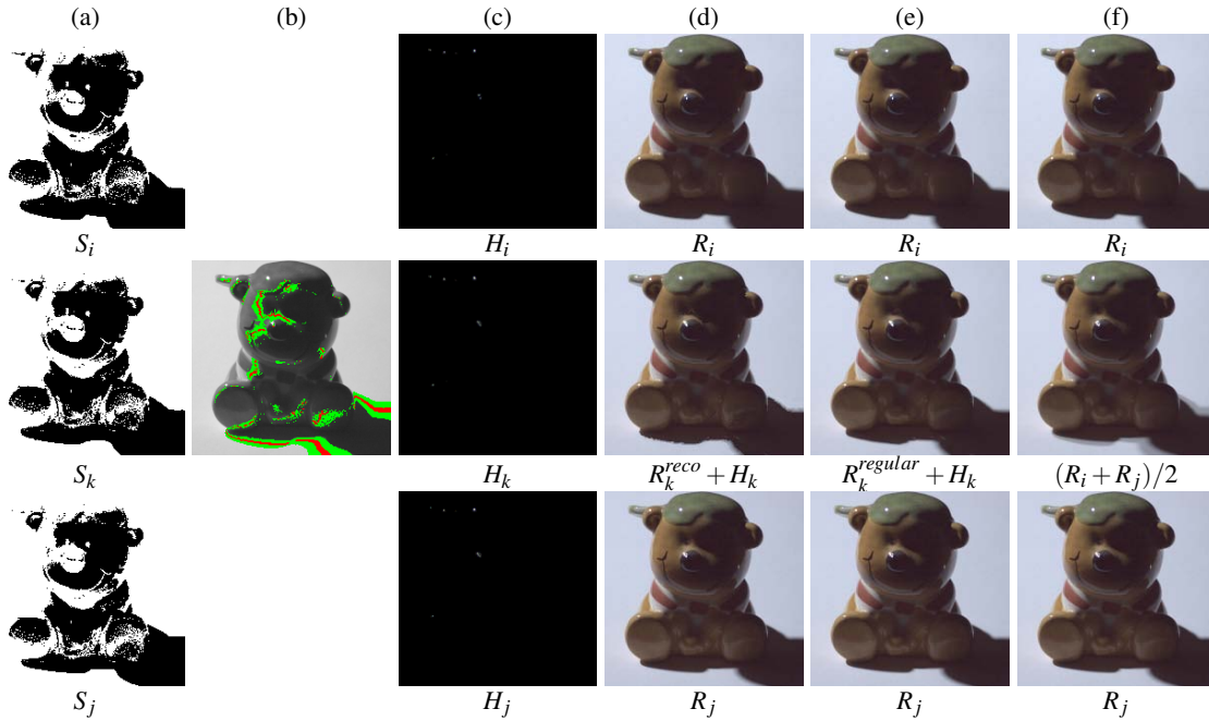
Figure 6: Illustration of the reconstruction process. The bottom and top row contain information from the initial, sparse input field. The in-between row is synthesized. By analyzing the shadow maps (a) we can obtain areas (b) where we either can locally interpolate (gray) or need to locally extrapolate (green and red). The green area is predicted to be fully lit or fully shadowed, the red area is the estimated location of the shadow boundary. After adding the highlight map (c), reconstruction yields a rough picture (d) which is improved using image-based priors (e). Especially the shadow boundary is much more pleasing than in a direct linear interpolation (f).
