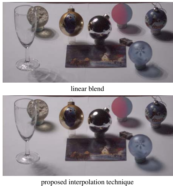
Figure 1: Relighting a sparsely sampled reflectance field (230 input images) with a small area light source. Top: Linear interpolation of the input samples results in banded shadows and disconnected highlights. Bottom: Our novel interpolation technique upsamples the same input reflectance field, effectively increasing its resolution to 3547 samples, and is capable of plausibly reproducing smooth shadows, shadows of semi-transparent objects, highlights and caustics.
