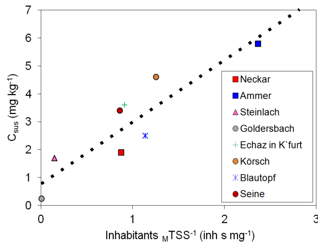
Fig. 2.6: PAH concentrations on suspended particles ( C_{sus} ) versus inhabitants normalized by the mean sediment mass yield ( \text{Inhabitants}_{MTSS^{-1}} ); adapted from Schwientek et al., 2013 (see also Schwientek 2017).
