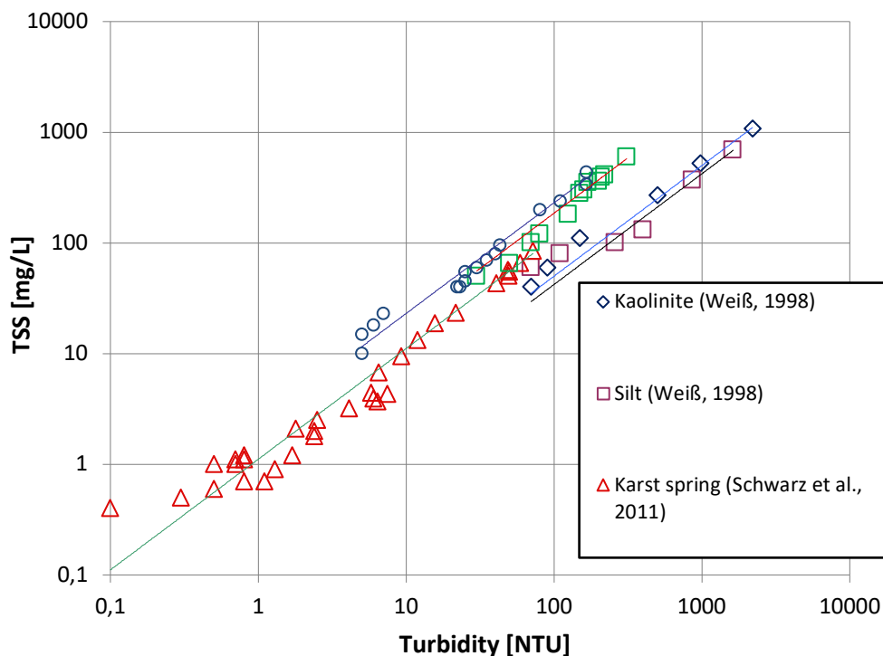
Fig. 2.1: Correlations of total amount of suspended solids (particles > 0.45 µm) to turbidity measured with light scattering (NTU); from Schwientek et al. (2013).
