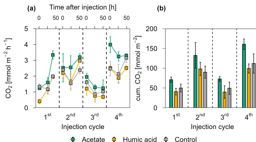
Figure 4. CO 2 release over four OC injection cycles for the acetate, humic acid, and control plots in the pioneer marsh. The dashed lines separate the individual injection cycles. (a) presents individual measured CO 2 fluxes 1.5, 24, and 48 h after injection in CO 2 mmol m -2 h -1 . Acetate (green), humic acid (orange), and NaCl for the control (grey) were injected into the sediment and GHG fluxes were measured directly above the injection spot at the aforementioned time intervals. (b) shows the cumulative CO 2 emissions in CO 2 mmol m -2 over one injection cycle for each treatment and control. We note here that some variability in the fluxes based on factors such as day/night could not be captured in our sampling approach; we therefore aimed to use a consistent approach and report relative changes rather than emphasize absolute values. For (a) and (b), markers represent mean \pm standard error of triplicates for all treatments and the control across injection cycles. For the 1st and 3rd injection cycle for the acetate treatment (both 1.5 h values) were based on duplicate measurements, which is thus also the case for the (b) cumulative CO 2 emission of these cycles.
