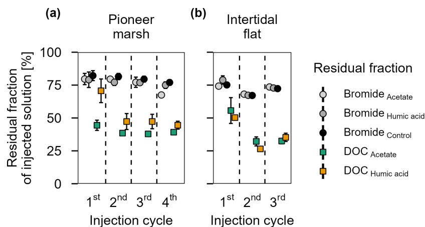
Figure 3. Residual fraction of injected solutions (Br - and DOC) in percentage after 48 h for treatments (acetate, humic acid) and control plots in the (a) pioneer zone (over four injection cycles) and (b) intertidal flat (over three injection cycles). Coloured squares show the residual fraction of injected DOC (acetate in green and humic acid in orange). The grey shaded circles represent the residual of Br - from the different treatments and the control. The values were calculated based on the ratio between the measured DOC or Br - concentration (porewater concentration 48 h post injection) and the expected DOC or Br - concentration (native + added). Markers represent the mean of the triplicates, with error bars indicating the corresponding standard error for treatments and control in both zones for DOC and Br - across all injection cycles.
