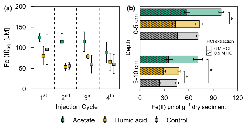
Figure 5. Ferrous iron in (a) porewater and (b) solid phase from acetate and humic acid treated plots and the control plots in the pioneer marsh. (a) Aqueous ferrous iron ( \text{Fe(II)}_{\text{aq}} ) [ \mu\text{M} ] sampled after each injection cycle (cycles are separated by the dashed line). Triplicates for each treatment and control for each injection cycle were collected and mean \pm standard error is shown. (b) HCl extractable \text{Fe(II)} content [ \mu\text{mol g}^{-1} dry sediment] at two different depths (0–5 and 5–10 cm) sampled at the end of all four injection cycles. Different colour coding was used for contrasting treatments: acetate treatment (green), humic acid treatment (orange), and control (grey). Striped bars represent poorly crystalline \text{Fe(II)} (0.5 M HCl extraction) and solid bars higher crystalline \text{Fe(II)} (6 M HCl extraction). The 0.5 M HCl extract was subtracted from the 6 M HCl extracted fraction to separate poorly and higher crystalline \text{Fe(II)} . Significance is denoted for the 0.5 M HCl extraction. Statistical details are given in the Supplement (Table S11), significance level * p < 0.05 . For each treatment and control, each spatial triplicate ( n = 3 ) was analyzed in triplicate (total n = 9 ) for each depth (0–5 and 5–10 cm); results are presented as mean \pm standard error.
