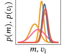
Figure 3.6.: Gaussian Approximation of the maximum of Gaussian distributed variables. The blue and red lines show Gaussian approximations to the maximum m of three independent Gaussian variables v_1, v_2, v_3 plotted in yellow (—). The approximation plotted in blue (—) includes a Gaussian prior (—) for the maximum. The red one (—) is obtained if no prior information on the maximum is included.
