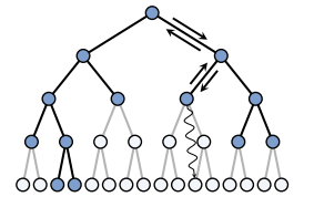
Figure 2.5.: An iteration during Monte Carlo Tree Search.
