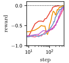
Figure 5.4.: Performance on Tic-Tac-Toe of PDAGS (—) and PDAGS with softmax values (—) with UCD (—) and UCT (—) and PTS (—). All methods obtain the optimal reward (---) in the end. Average reward from 20 search runs. Standard deviations over 25 such repetitions (of 20 runs) as shaded regions.
