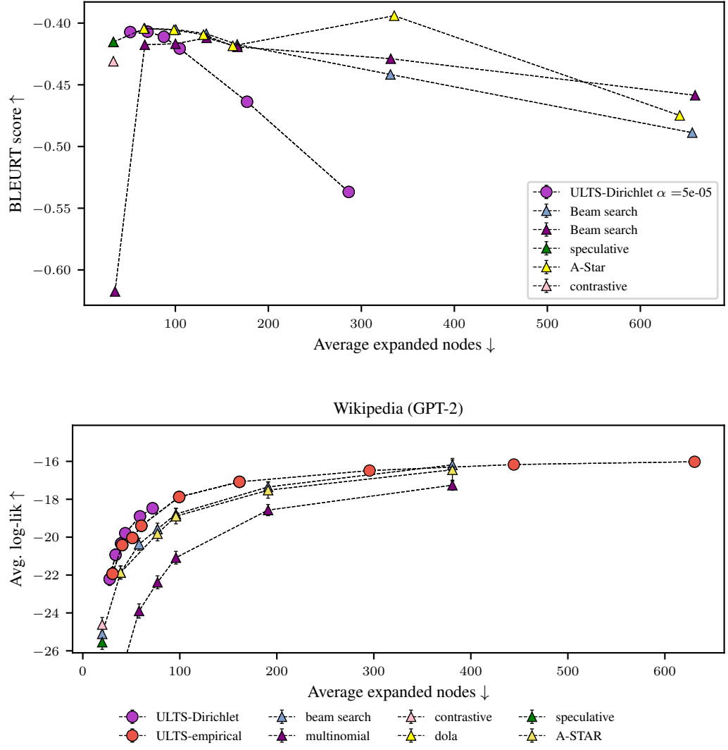
Figure D.12.: Comparison of ULTS with the baselines on the Wikipedia dataset as described in Section 6.5 with additional data points for k_{\max} \in \{50, 100, 200\} .
