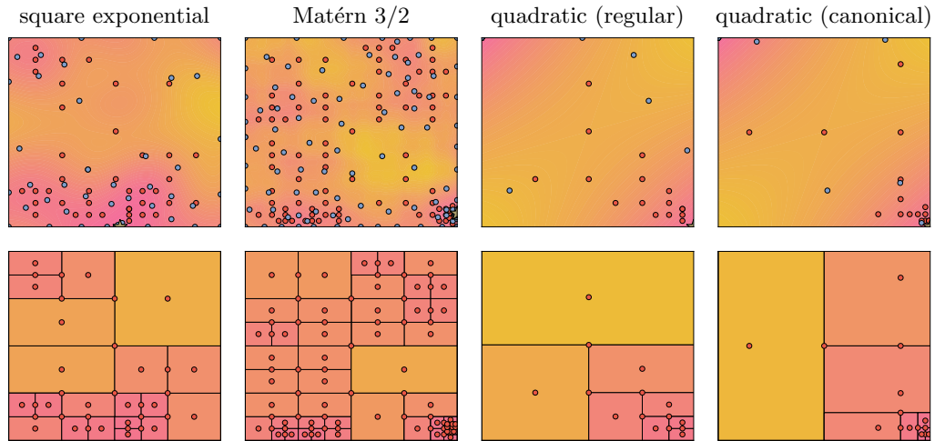
Figure 4.1.: Top: Sample from a Gaussian process and evaluation locations of GP-OO \bullet and GP-UCB \circ . More pink colors indicate higher function values. \star marks the optimal function value. On the examples here they all happen to lie on the boundaries of the domain. Bottom: Cells and diameters \Delta . More pink colors indicate smaller diameters.
