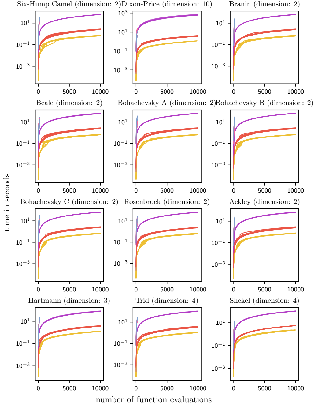
Figure B.3.: Cumulative run-times for common benchmark datasets. GP-OO is shown in — , GP-UCB in — , EI in — , DIRECT in — , TURBO in — and random selection in — . Averages in bold.
