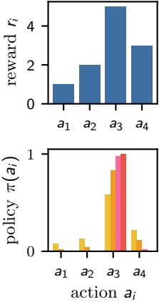
Figure 3.3.: The softmax of a reward function. Top: Rewards for k = 4 arms. Bottom: The softmax distribution over the arms for four different values of the parameter \beta :
