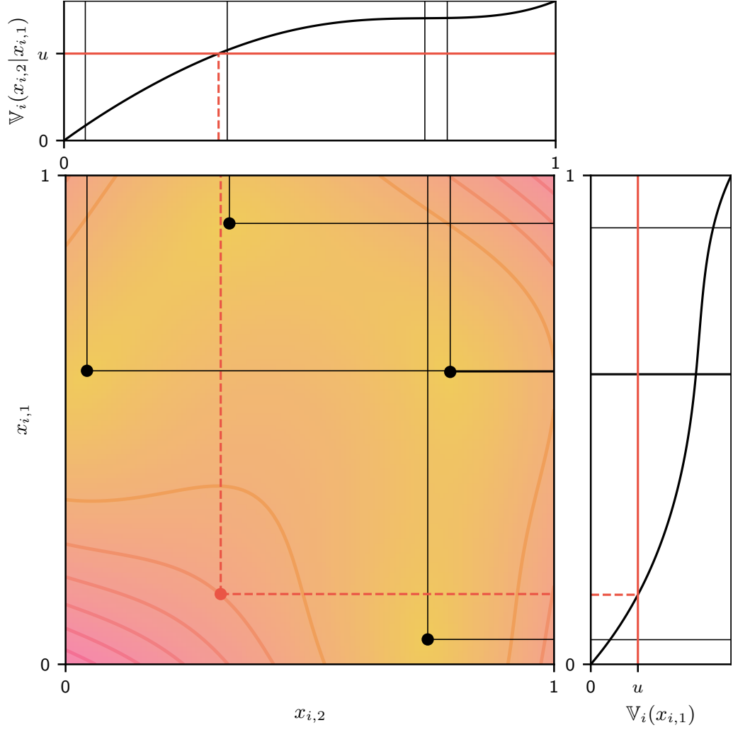
Figure 7.3.: Drawing approximate k -DPP samples in two dimensions. Bottom left: Contour plot of the multivariate probability density \text{Var}_i(x) with (i = 5) ; preceding four samples as black points. Right: The first coordinate of the fifth sample is drawn first, from the marginal density along this dimension. Top: The second coordinate is then drawn by computing a cumulative density conditioned on the value of the first coordinate.
