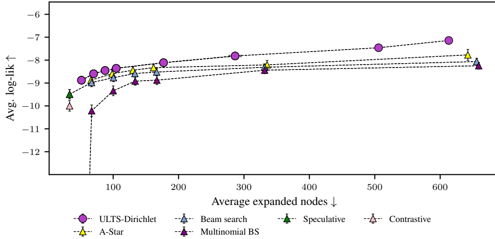
Figure D.13.: Comparison of ULTS in the machine translation task as described in Section 6.5 with additional data points for k_{\max} \in \{50, 100\} .
