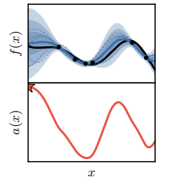
Figure 3.4.: GP-UCB. Top: Objective function (—) with six noisy function evaluations (●). The posterior mean and variance (—) and posterior samples (---) of the Gaussian process are also shown. Bottom: GP-UCB acquisition function (—). The star (★) marks the next evaluation point.
