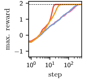
Figure 5.3.: Performance on synthetic search problems of PDAGS (—) and PDAGS with softmax values (—) with UCD (—) and UCT (—). All methods obtain the optimal reward (---) in the end. Shaded regions show standard deviations from 500 runs each.
