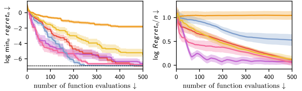
Figure 4.3.: Best simple regret (left) and cumulative regret (right) on synthetic functions sampled from a Gaussian process. GP-OO is shown in red, GP-UCB in blue, EI in pink, DiRect in yellow, TURBO in purple and random selection in orange. Averages and standard error of the mean from 20 runs.
