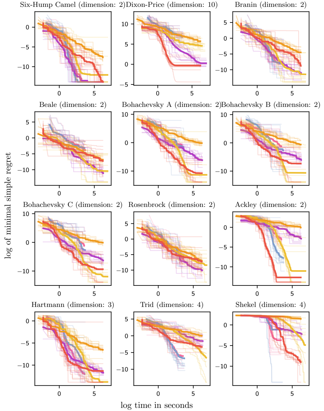
Figure B.1: Minimal simple regret obtained on common benchmark datasets for simulated function evaluation costs of 0.1 Second. GP-OO is shown in red, GP-UCB in blue, EI in pink, DIRECT in yellow, TURBO in purple and random selection in orange. Averages in bold.
