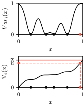
Figure 7.2.: Sketch illustrating analytic sampling from a k -DPP in one dimension, using the square-exponential kernel (Equation 7.22). Top: Posterior variance \text{Var}_i(x) after the 4th iteration ( i = 5 ). Bottom: Inverse transform sampling from \text{Var}_i(x) , by computing the cumulative density \mathbb{V}_i (black line), drawing a scaled uniform random sample u and finding the point x_i such that \mathbb{V}_i(x_i) = u , by interval bisection.
