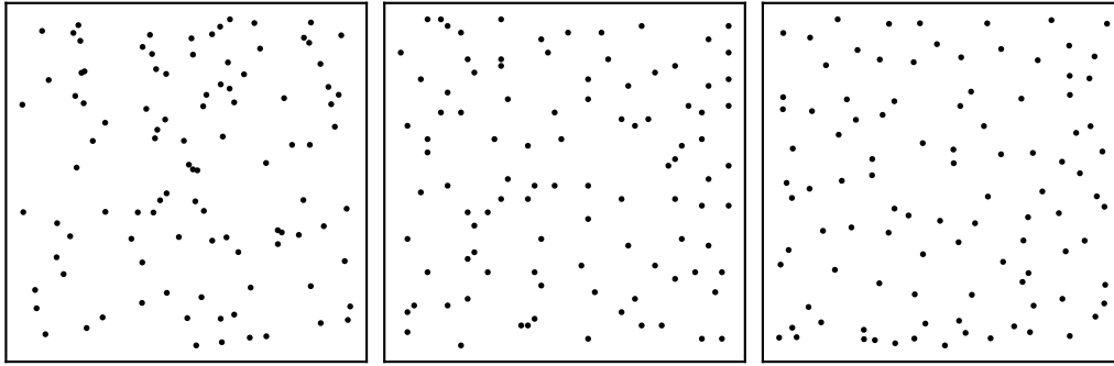
Figure 7.1.: 100 random points on the interval [0, 1]^2 sampled uniformly at random ( left ), sampled from a k -DPP with square-exponential kernel with a length-scale of 0.1 ( middle ), and sampled from its greedy approximation that is the subject of this paper ( right ).
