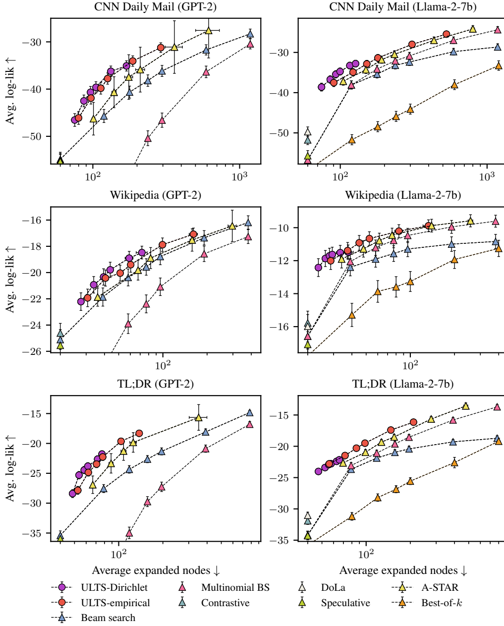
Figure 6.4.: Decoding experiments with Llama-2-7b and GPT-2 for text generation on CNN Daily Mail and Wikipedia articles and text summarization for the TL;DR dataset. The methods are evaluated for different computational budgets, i.e. different values of k and k_{\max} . ULTS dominates the baselines in low-budget settings. Errorbars indicate two times the standard error of the mean.
