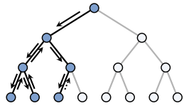
Figure 2.1.: Depth-First Traversal explores as far down a branch as possible before backtracking to explore other branches.
