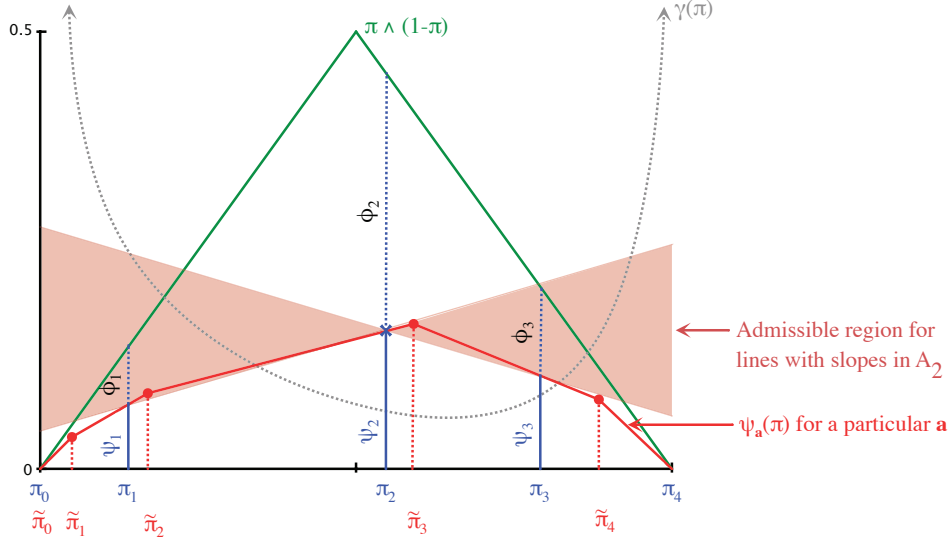
Figure 8: Illustration of construction of optimal \psi(\pi) = \mathbb{L}(\pi, P, Q) . The optimal \psi is piecewise linear such that \psi(\pi_i) = \psi_i , i = 0, \dots, n+1 .
