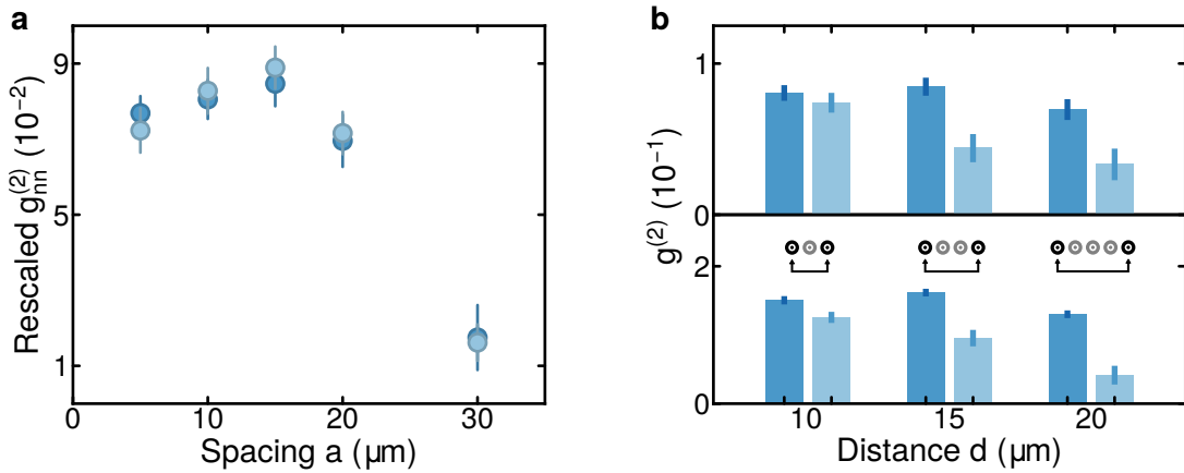
Figure 4.17: Two-body correlation as a function of the array spacing and with ponderomotive barriers. a Next-neighbour correlation g_{nm}^{(2)} in a 1D chain of traps versus the spacing of the traps a . Measurement done for detuning \Delta = -2\pi \cdot 2 \text{ MHz} dark blue dots and \Delta = -2\pi \cdot 5 \text{ MHz} light blue dots. The correlation amplitude is scaled globally to the same average amplitude. b Histograms for \Delta = -2\pi \cdot 2 \text{ MHz} on top and \Delta = -2\pi \cdot 5 \text{ MHz} at the bottom, showing the effect of a ponderomotive barrier between two tweezers, see illustration in the figure. The dark blue bars correspond to the case of no ponderomotive barrier in between the tweezers at the respective distance. The light blue bars instead correspond to the case with at least one barrier in between. The correlation is calculated on a subset of the data through post-selection. The data in the light blue columns was postselected in a way that the tweezers in between the set distance were empty after the initial loading of the array. Error bars denote 1 s.e.m.
