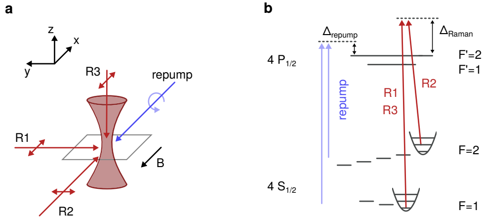
Figure 3.26: Beams dispositions and level diagram for Raman sideband cooling. a Schematic of the Raman beams with respect to the traps. We apply a quantization field of 1.5 \text{ G} along the x -axis. The repumpers are circularly polarized to drive \sigma^+ transitions. All the Raman beams are linearly polarized to prevent the generation of vector light shifts. R1 and R2 lie on the x - y plane and only couple radial sidebands. R3 is aligned along the z -axis and, together with R2, addresses the axial sidebands. b Level scheme for the Raman sideband cooling. The Raman laser drives transitions between the F = 2, m_F = +2, n and the F = 1, m_F = +1, n - \Delta n states. The Raman laser is blue detuned by 40 \text{ GHz} with respect to the D1 line. The repumper light is detuned \approx 2\pi \cdot 80 \text{ MHz} from the D1 line to reduce the heating from the anti-trapped excited states. Figure from [62].
