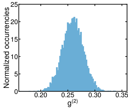
Figure 1: Re-sampling distribution. Distribution of the calculated two-body correlation g^{(2)} from real experimental data with the application of the resampling method. The two-body correlation is calculated by randomly sampling the experimental data. Each sample has the same size of the experimental data and can contain several copies of the data. The sample is formed by selecting with a uniform random distribution the data. N = 10^3 resamplings were made to produce the histogram in the figure.
