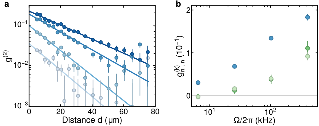
Figure 4.18: Avalanche facilitated excitation. a Two-point correlations g^{(2)} vs. distance for different coupling strength in a 3 \times 16 array with 5 \mu\text{m} spacing. The Rabi coupling is increased from light to dark blue as \Omega = 2\pi \cdot (6, 25, 102, 410) kHz with the pulse time adjusted to fix the fraction of lost atoms at 20%. Exponential fits are shown as solid lines. b Multi-point correlations vs. coupling strength. The values are plotted for the shortest distance connected multi point correlations g_{n..n}^{(k)} along the x-axis. The correlations are shown for k = 2 in blue, k = 3 in light green and k = 4 in dark green. Error bars denote 1 s.e.m.
