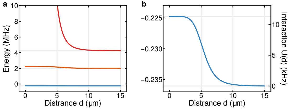
Figure 4.3: Rydberg dressing interaction. a Eigenenergies for the pair-state forming the base for the interaction Hamiltonian as a function of the inter atomic distance. The blue line shows the eigenenergies for |gg\rangle , orange for |+\rangle and red for |rr\rangle . Establishing a realistic value for the coupling \Omega = 2\pi \cdot 1 MHz and detuning \Delta = -2\pi \cdot 2 MHz, we will consider an interaction strength of C_6 = 100 GHz \mu\text{m}^6 . b Zoom on the resulting shift for the ground pair-state |gg\rangle showing the characteristic soft core potential with a soft core radius r_c = 5.4 \mu\text{m} . The overall shift to negative eigenenergies is given by the AC stark shift \delta_{AC} .
