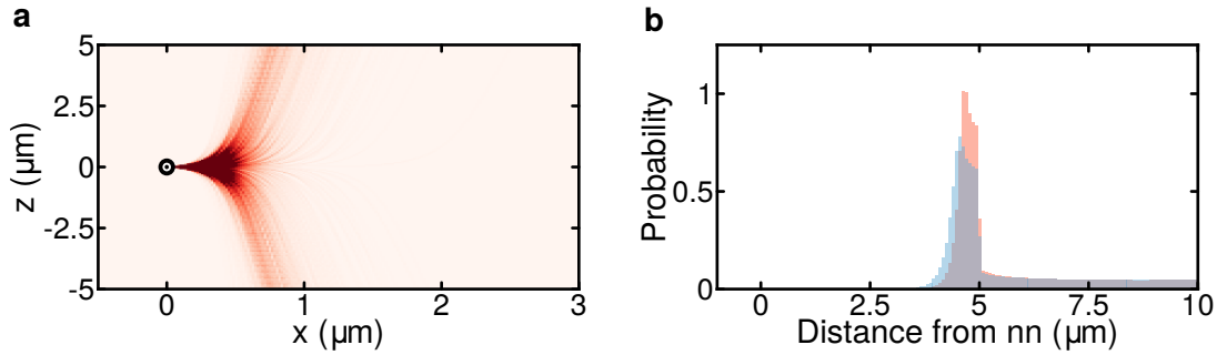
Figure 4.20: Removal of excited atoms. a Density plot of the trajectories obtained with a classical Monte-Carlo simulation for the motion of one Rydberg atom. In the simulation, we consider a single tweezer that propagates along the z -axis and an elliptical light beam with w_z = 3 \mu\text{m} and w_x = 50 \mu\text{m} that can be used as a dipole trap for the atoms in the ground state. The Rydberg atom sees a repulsive potential from the tweezer U_{twe} = 2\pi\hbar \cdot 77 \text{ kHz} and one from the elliptical dipole trap beam of U_{dip} = 2\pi\hbar \cdot 20 \text{ MHz} . The atom receives a kick from the absorbed UV photon and has an initial velocity from its temperature as in the simulation in Section 4.3.4 . We can see that the atoms are quickly accelerated away from the atomic plane in the vertical direction. If we consider an array spacing of a = 5 \mu\text{m} we can see that the atom is not able to reach its nearest neighbor compared to the simulations shown in Fig. 4.15 . b We plotted the histogram of the normalized distribution of the sampled distances calculated between the moving atoms and the nearest-neighbor position. The atom starts at a 5 \mu\text{m} distance from the nearest neighbor. The red histogram is done with simulation for a repulsive potential of the dipole beam of U_{dip} = 2\pi\hbar \cdot 20 \text{ MHz} , the blue one is for U_{dip} = 2\pi\hbar \cdot 10 \text{ MHz} . In both cases, the atoms are not able to reach the neighbor position, and the distance increases quickly.
